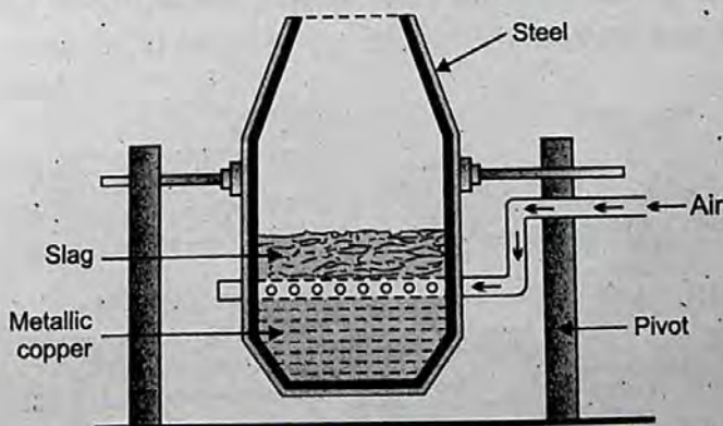
Fig. 16.5 Bessemer converter used for bessemerization of copper.
