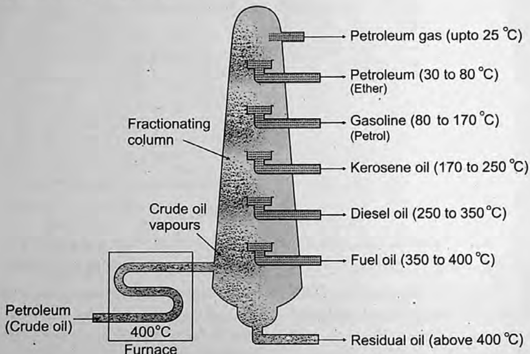
Fig 16.11 Fractional distillation of petroleum.
