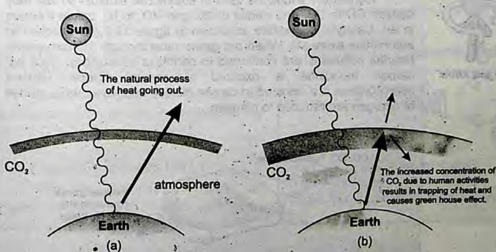
Fig. 14.3 Greenhouse effect.
