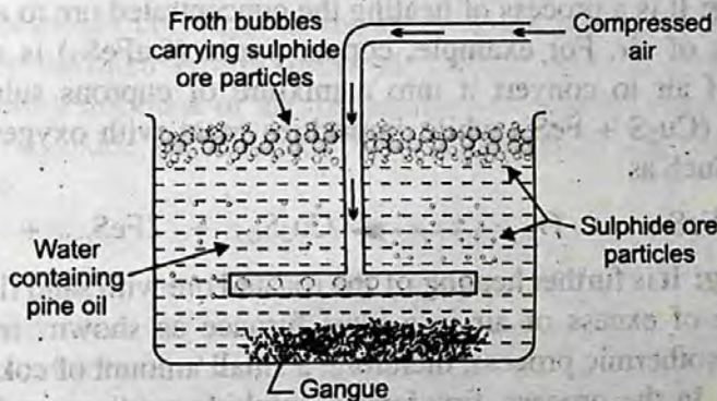
Fig. 16.2 Froth flotation process
