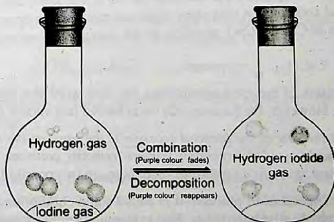
Fig. 9.1 Showing establishment of reversible reaction.
