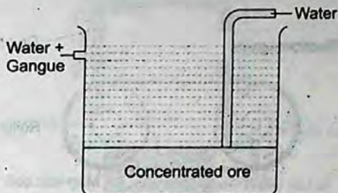
Fig. 16.1 Gravity separation
