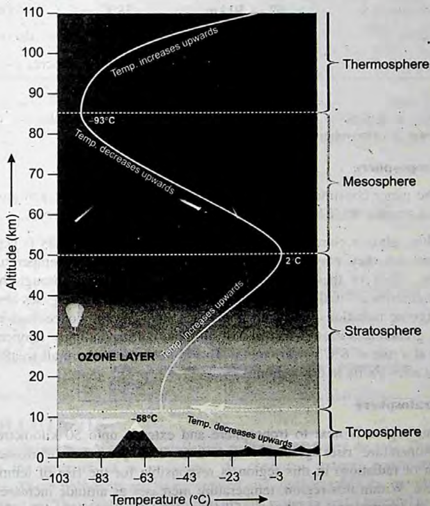
Fig. 14.1 Different spheres of atmosphere.
