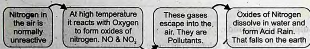
Fig. 14.7 Formation of NO & NO 2 on combustion of fossil fuel and causing air pollution.
