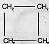
Cyclobutane
