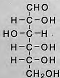
Glucose
