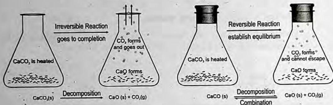
Fig. 9.2 Showing establishment of reversible reaction.
