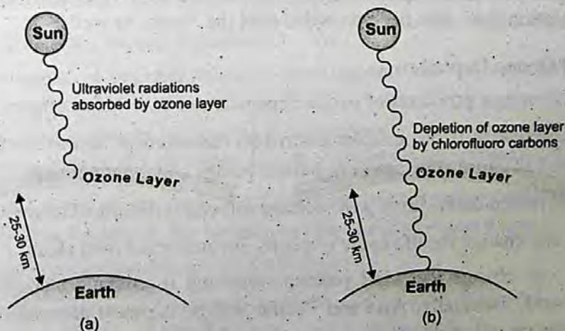
Fig. 14.10 (a) Ozone layer (b) Depletion of ozone layer.
