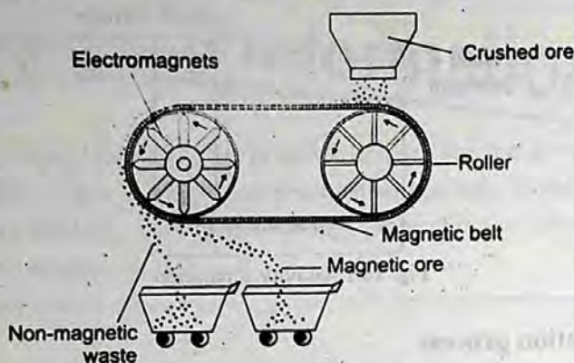
Fig 16.3: Magnetic separation
