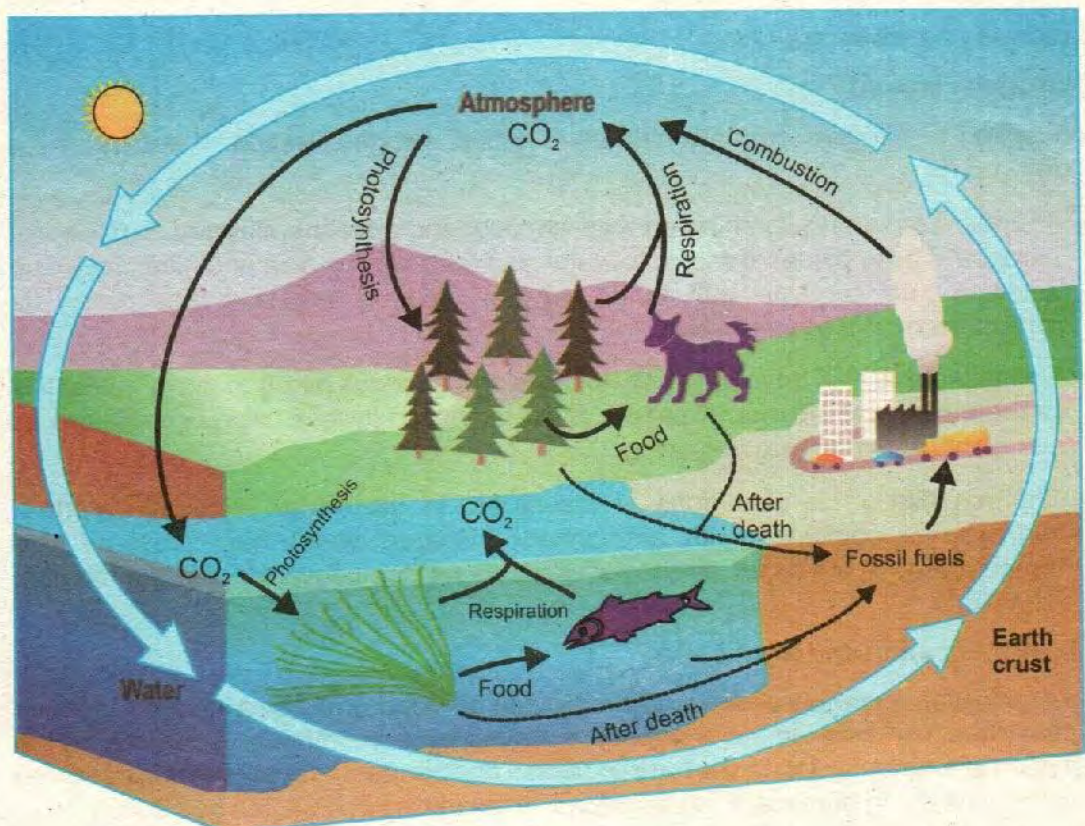
Figure 16.7: Carbon cycle
